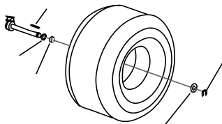
Fig. 29 — Remover a roda
